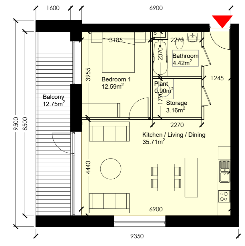
Unit Type 1B_02 Scale 1:100 @ A0
