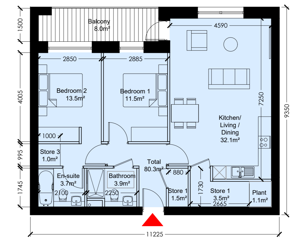
Unit Type 2B_01 Scale 1:100 @ A0
