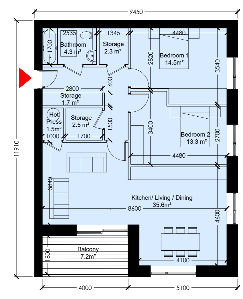
Unit Type 2B_09 Scale 1:100 @ A0
