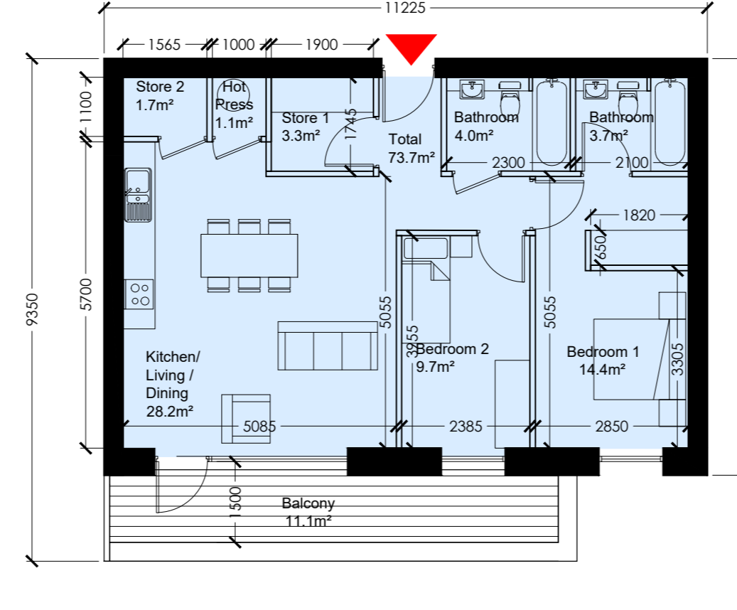
Unit Type 2B_05 Scale 1:100 @ A0
