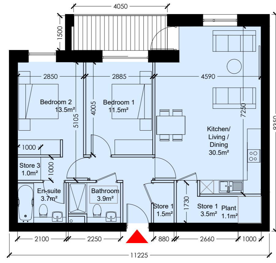
Unit Type 2B_04 Scale 1:100 @ A0
