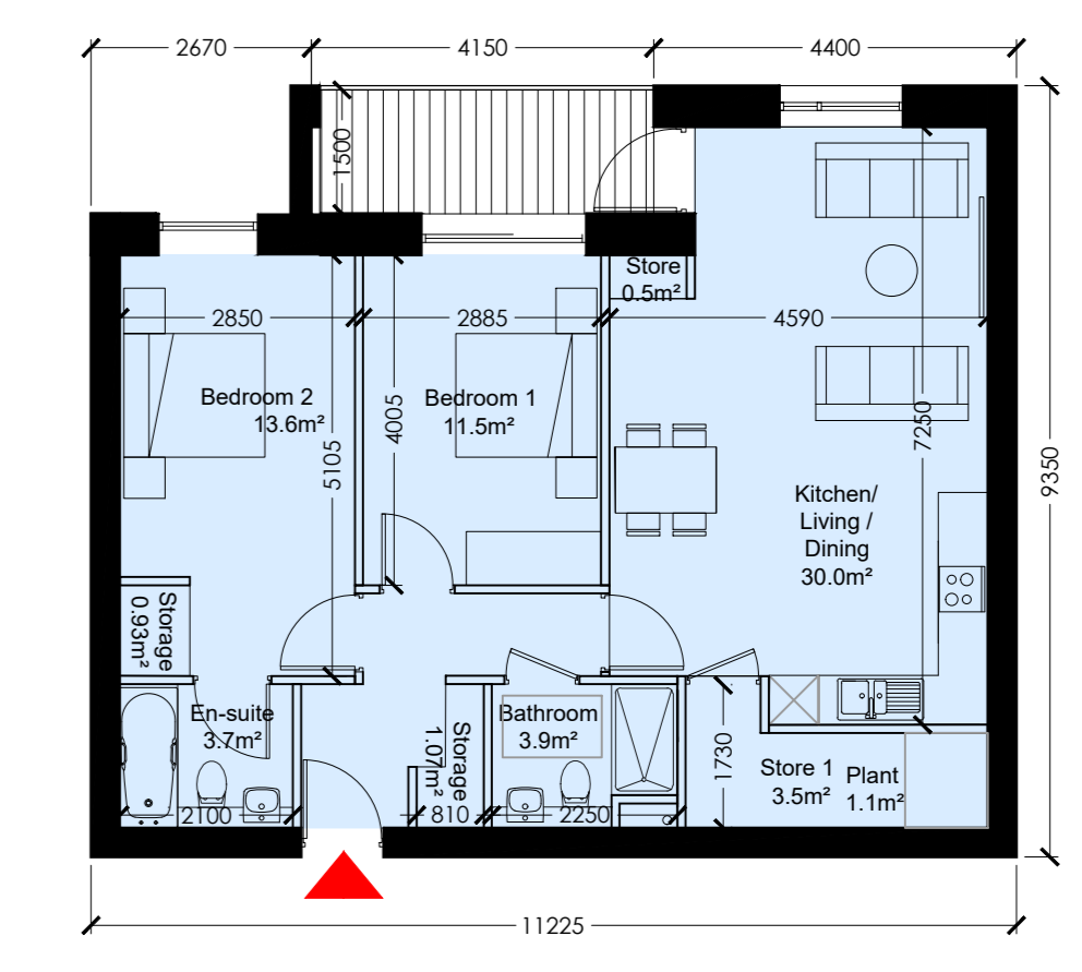
Unit Type 2B_10 Scale 1:100 @ A0
