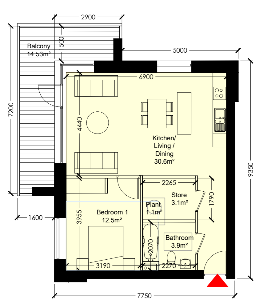
Unit Type 1B_01 Scale 1:100 @ A0
