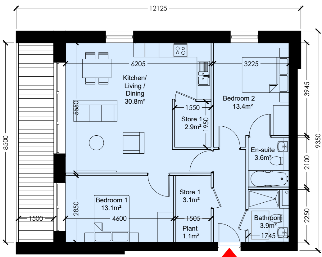
Unit Type 2B_03 Scale 1:100 @ A0
