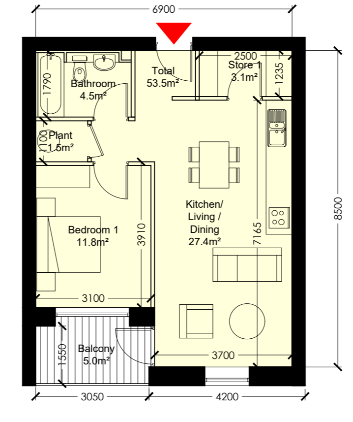
Unit Type 1B_03 Scale 1:100 @ A0
