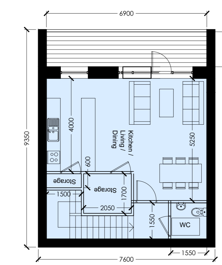
First Floor Level - 47.61 m 2
